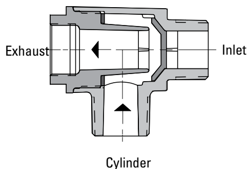
Valve Open to Exhaust
