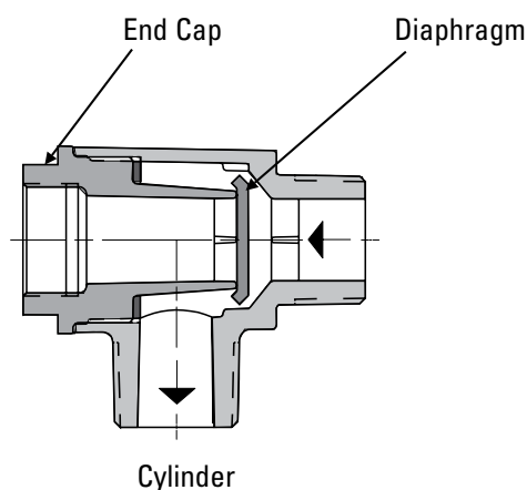
Valve Pressurized
