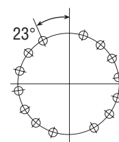
Pressure Plate Coolant Inlet Port 48WCSB 14-1.438 (36,5) Dia. Holes based on 16 Equally Spaced Holes on a 54.000" (1371,6) BC
