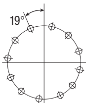
Pressure Plate Coolant Inlet Port 24WCSB 12-0.656 (16,7) Dia. Holes Equally Spaced Holes on a 28.750" (730,3) BC
