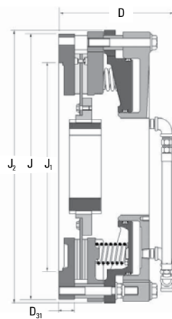
Single Disc Brake
