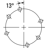
15DC (6) 0.656 (16.7) Ø Mounting Holes Based on 8 Equally Spaced as Shown on 17.500 (444.5) Bolt Circle
