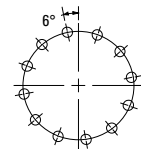
(12) 0.656 (16.7) Ø Mounting holes equally spaced as shown on 28.750 (730.3) Bolt
