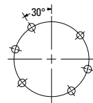
(6) 0.656 (16.7) Ø Mounting holes based on 8 equally spaced holes on 18.375 (466.7) Bolt
