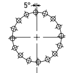
(16) 1.062 (27.0) Ø Mounting holes equally spaced as shown on 42.000 (1066.8) Bolt
