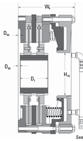
Dual Disc Brake
