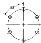
(6) 0.531 (13.5) Ø Mounting holes equally spaced as shown on 11.125 (282.5) Bolt
