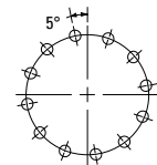
(12) 0.656 (16.7) Ø Mounting holes equally spaced as shown on 23.250 (588.8) Bolt
